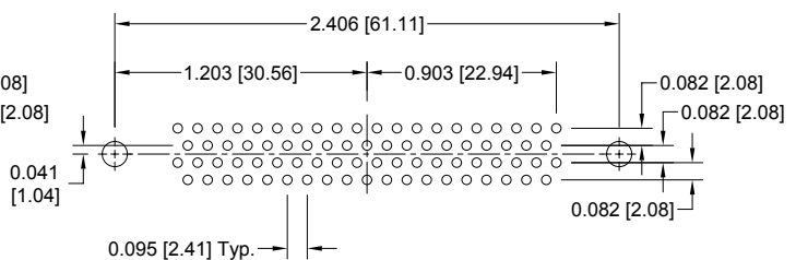
DD104 FEMALE
